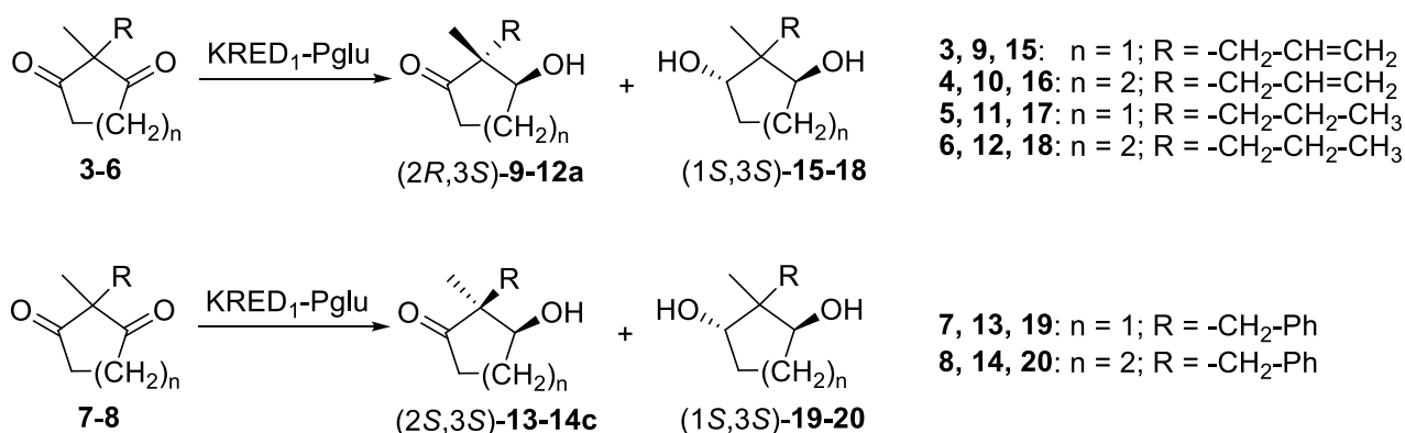
Scheme 4. Reduction of 2,2-disubstituted-1,3-cyclopentanediones and 1,3-cyclohexanediones with KRED1-Pglu.
